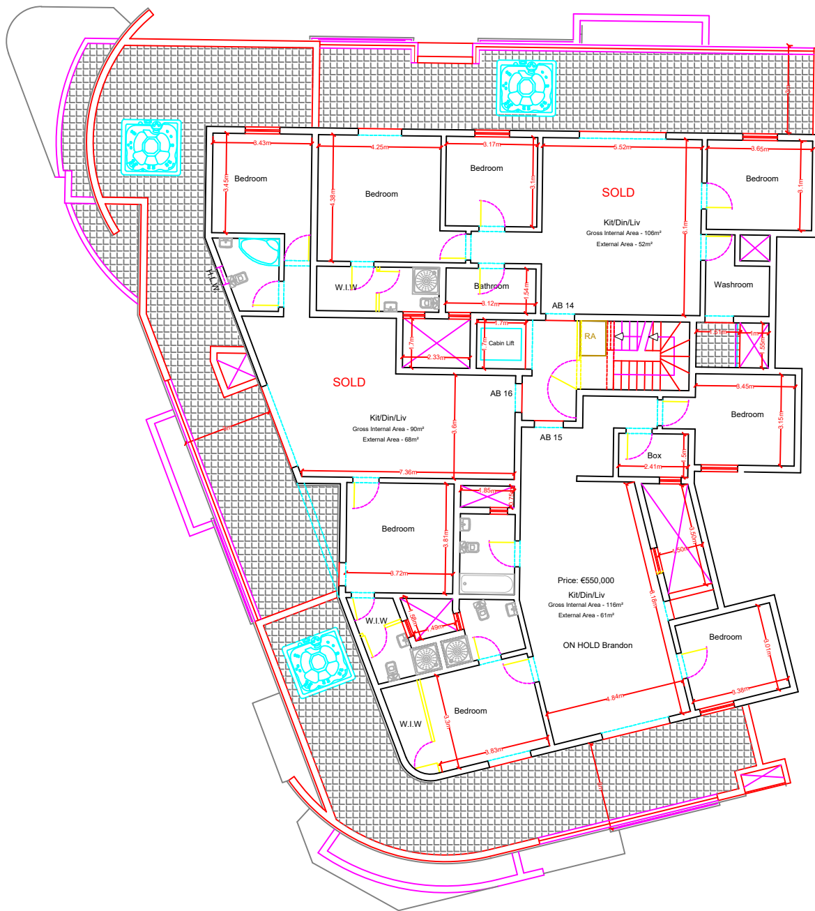
Approved/ Proposed Level 4 Scale 1:100
