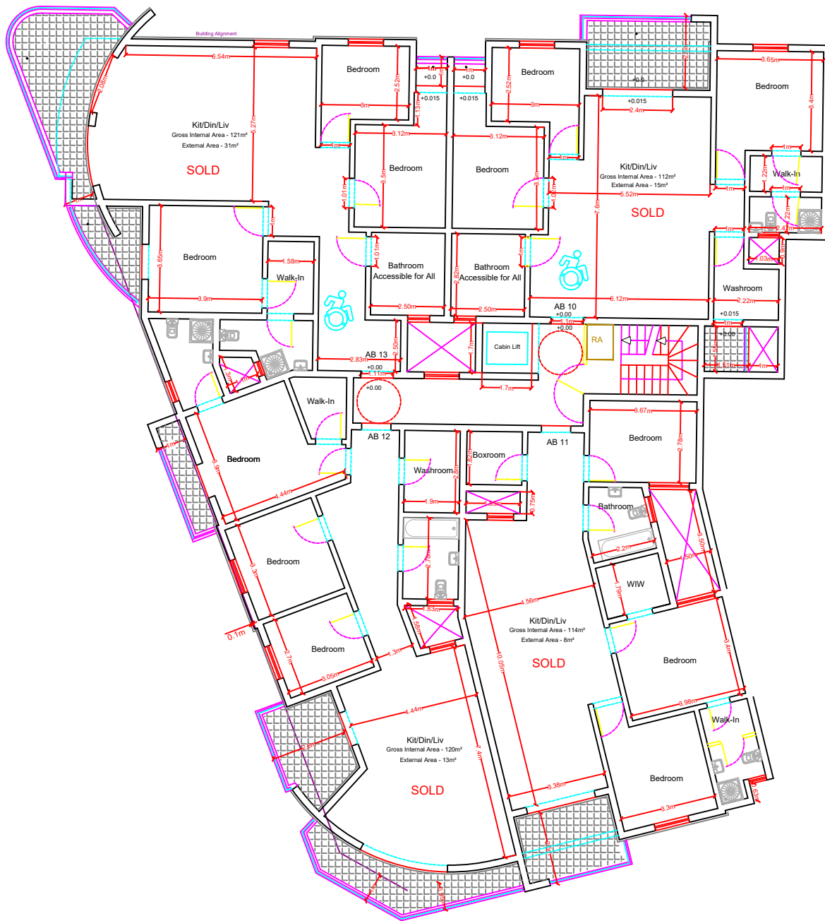
Approved/ Proposed Level 3 Scale 1:100
